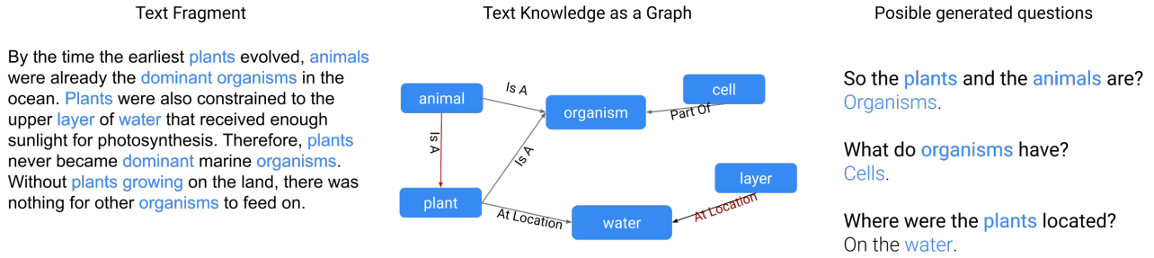
Figure 1: On the left, a text fragment with highlighted (on blue) entities related to biology extracted from WordNet Domains. On the middle, a handcrafted knowledge graph build from the triples proposed by the RE system (red edges denote incorrect triples). On the right, manually generated questions based on Olney et al. (2012) templates.
