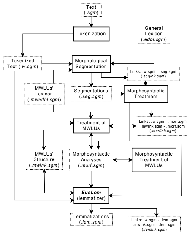
Figure 1. Detailed information flow between the analysis tools.
