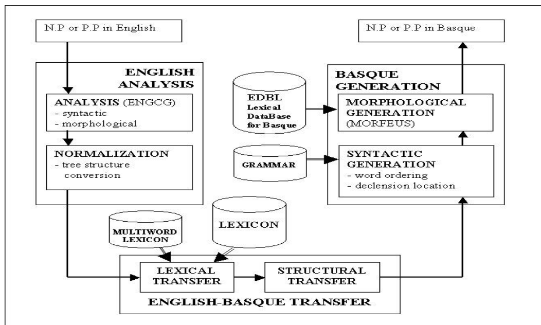
Figure 2. General architecture of the English-Basque modules
