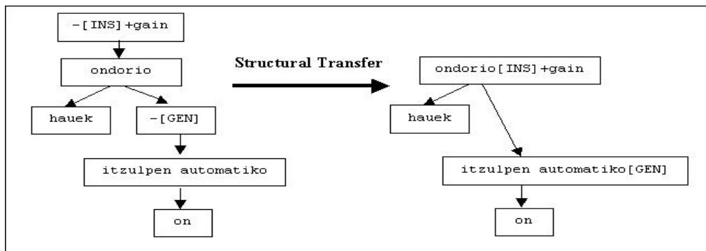
Figure 7. Structural Transfer
