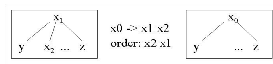
Figure 8. Structural Transfer
