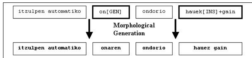
Figure 10. Morphological Generation
