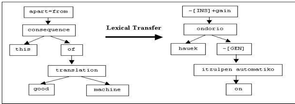
Figure 6. Lexical Transfer
