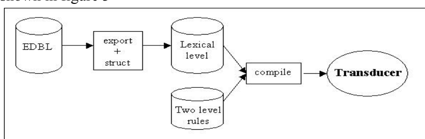
Figure 3. Building the transducer from the lexical database and two-level rules
