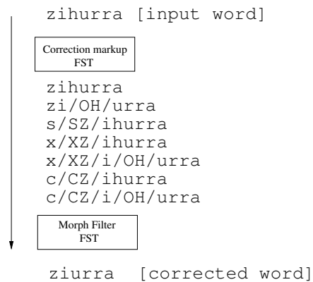
Fig. 1. An illustration of the functioning for the part of the spelling corrector that recognizes typical orthographical errors. A correction markup filter optionally changes the input to a number of possible candidate errors, after which the morphological filter retains only those that are actual words.
